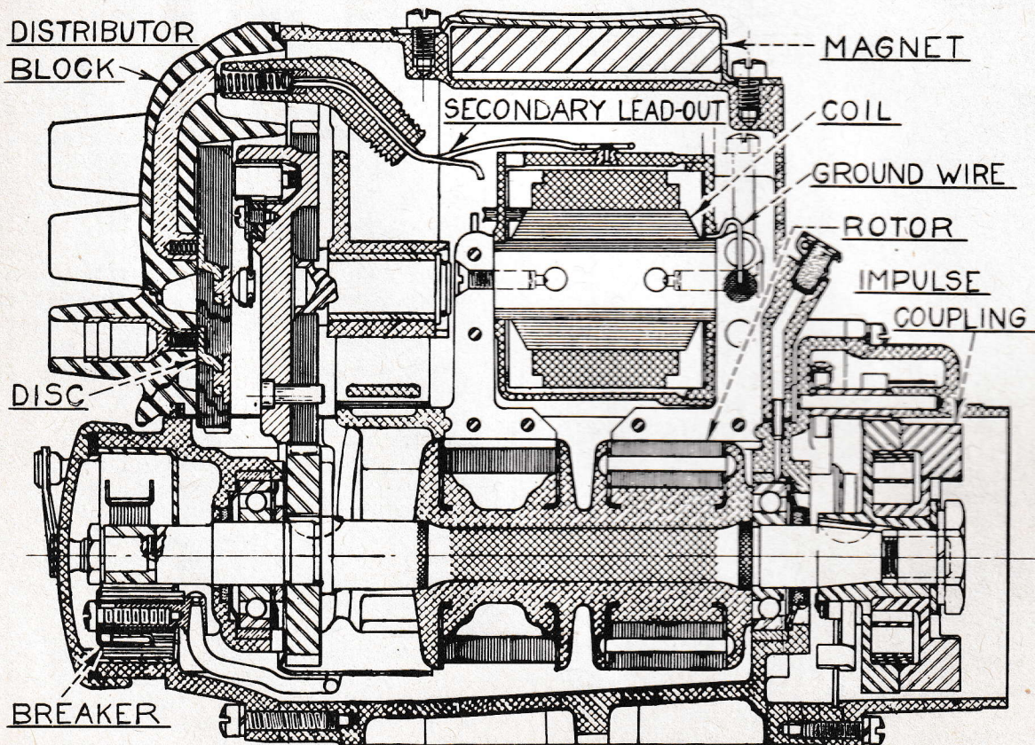
ILLUST. 7--CROSS SECTIONAL VIEW OF INTERNATIONAL F-6 MAGNETO.
