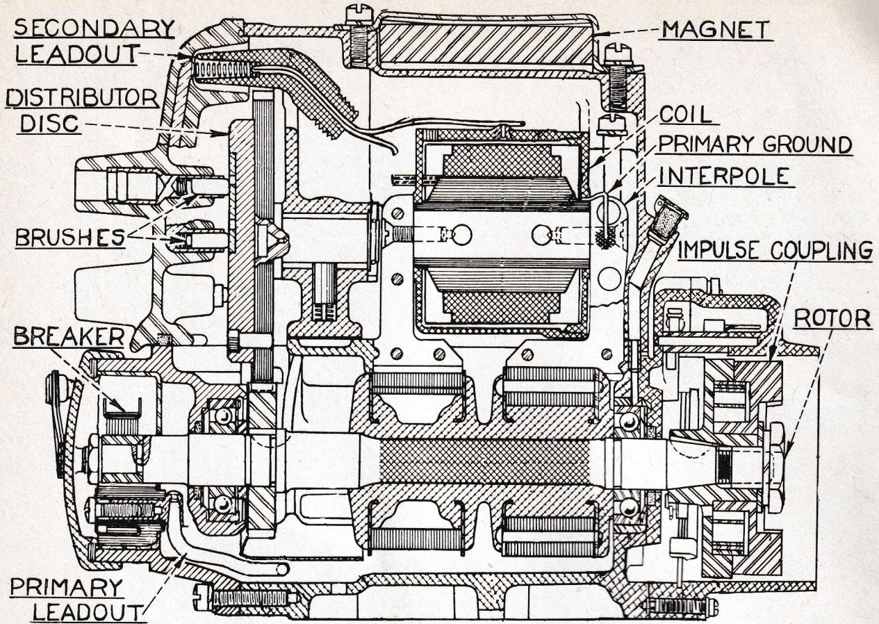
ILLUST. 6--CROSS SECTIONAL VIEW OF INTERNATIONAL F-4 MAGNETO.
